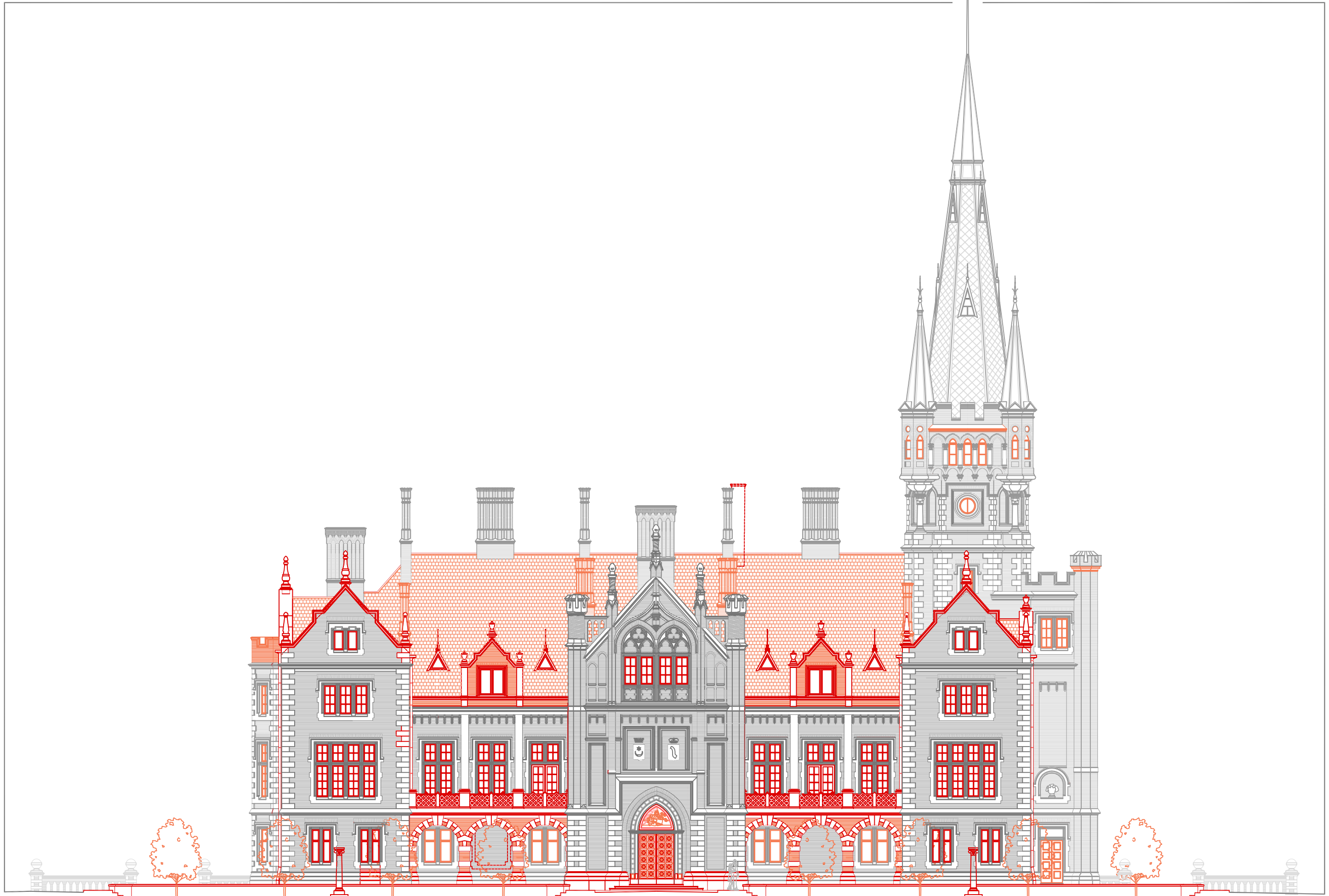
NORTHWEST ELEVATION
